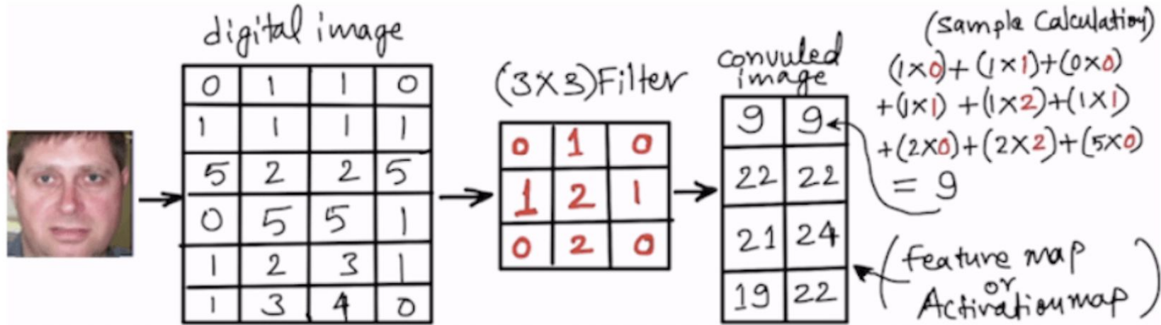
The Convolution step in CNN
